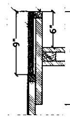
DETAIL-2
